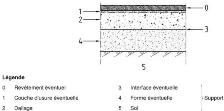
Figure 1 - Dallage
